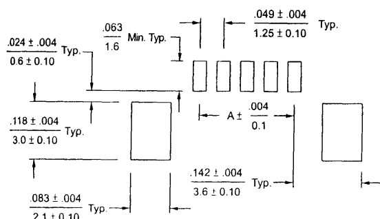
PCB Layout: Solider side
