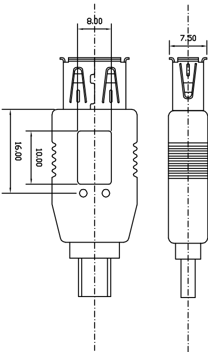
USB A FEMALE
