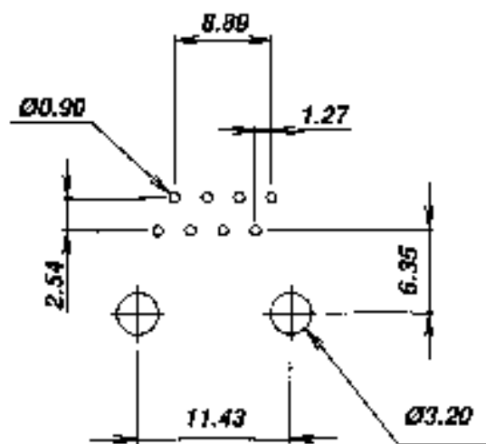
PCB LAYOUT
