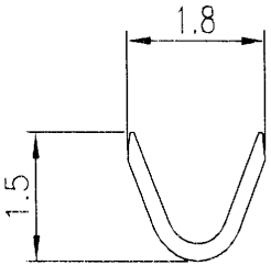
B-B SECTION
